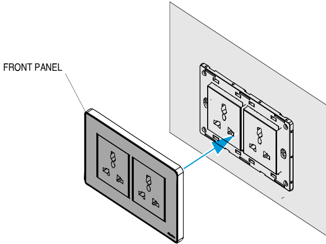
Figure 2B: Wiring Diagram - 2-Way Installation
